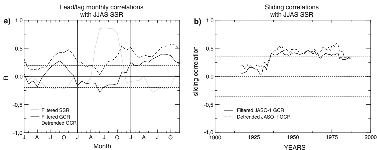
Fig. 7 a Lead–lag correlations between JJAS SSR in year 0 and monthly GCR anomalies from year -1 to year +1 (also shown are the auto–correlations with the filtered SSR timeseries). Note that the monthly timeseries have been filtered with a 5-month moving average to smooth the correlations that have been estimated
