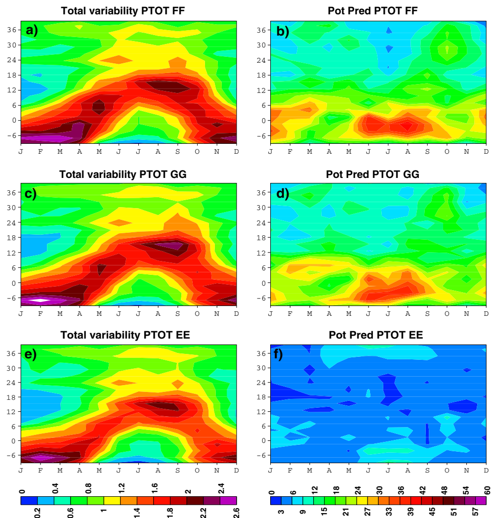
Fig. 10 Same as Fig. 9, but for precipitation
