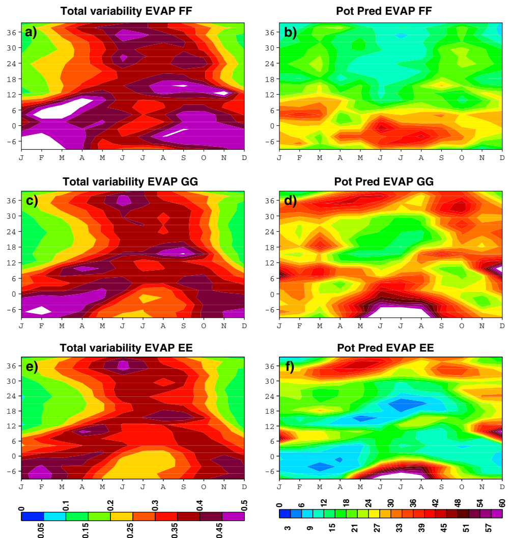
Fig. 9 Annual cycle of zonal mean (20°W–25°E) total variability ( left panels in mm/day) and potential predictability ( right panels in %) of surface evaporation over West Africa (land grid points only) between 10°S and 40°N
