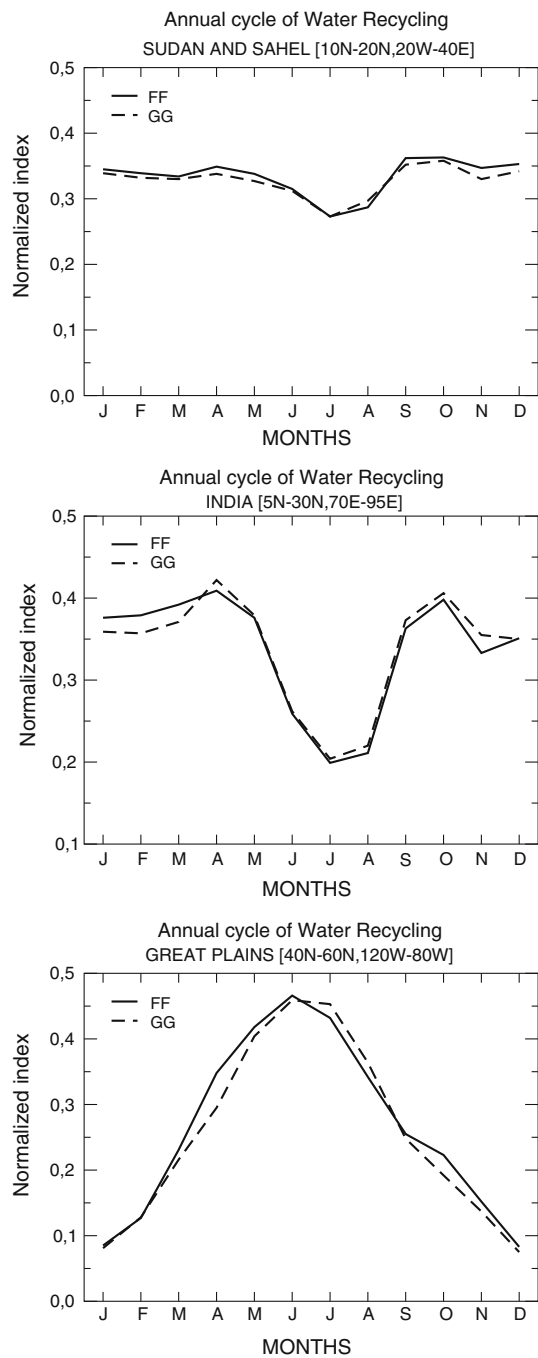
Fig. 14 Annual cycle of regional water vapour recycling ratio (see the text for details) in the FF and GG experiments over three regions, including sub-Saharan Africa ( top panel ), highlighted as “hot spots” in the GLACE intercomparison project
