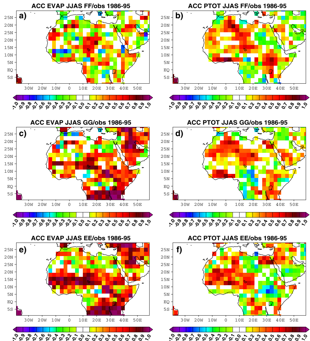
Fig. 11 Regional maps of temporal anomaly correlation coefficients (ACC) between simulated and analysed (GSWP2) or observed (CRU2) JJAS anomalies over the 1986–1995 period for surface evaporation ( left panels ) and precipitation ( right panels ), respectively
