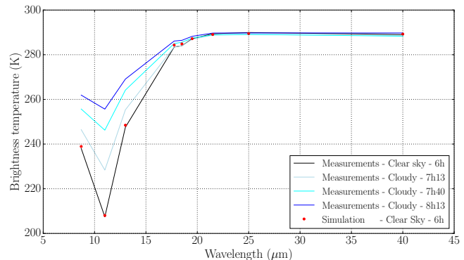
Figure 17. Brightness temperatures measured with the FIRR during the 2 July 2015 experiment. Four cases are shown with different cloud covers. They are also reported in Fig. 16. The MODTRAN simulation corresponding to the clear-sky conditions is indicated by red dots.
