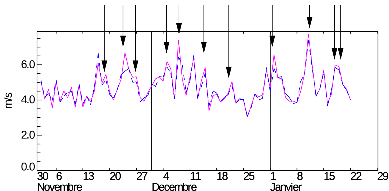
Figure 8: RMS of 24h forecasts of wind at 500 hPa over Europe, obtained from two different Arpège 4D-Var experiments. Pink full curve: with climatological ensemble sigma's. Blue dashed curve: with flow-dependent ensemble sigma's of the day. The vertical black arrows materialize the number of reductions of local RMS peaks.
