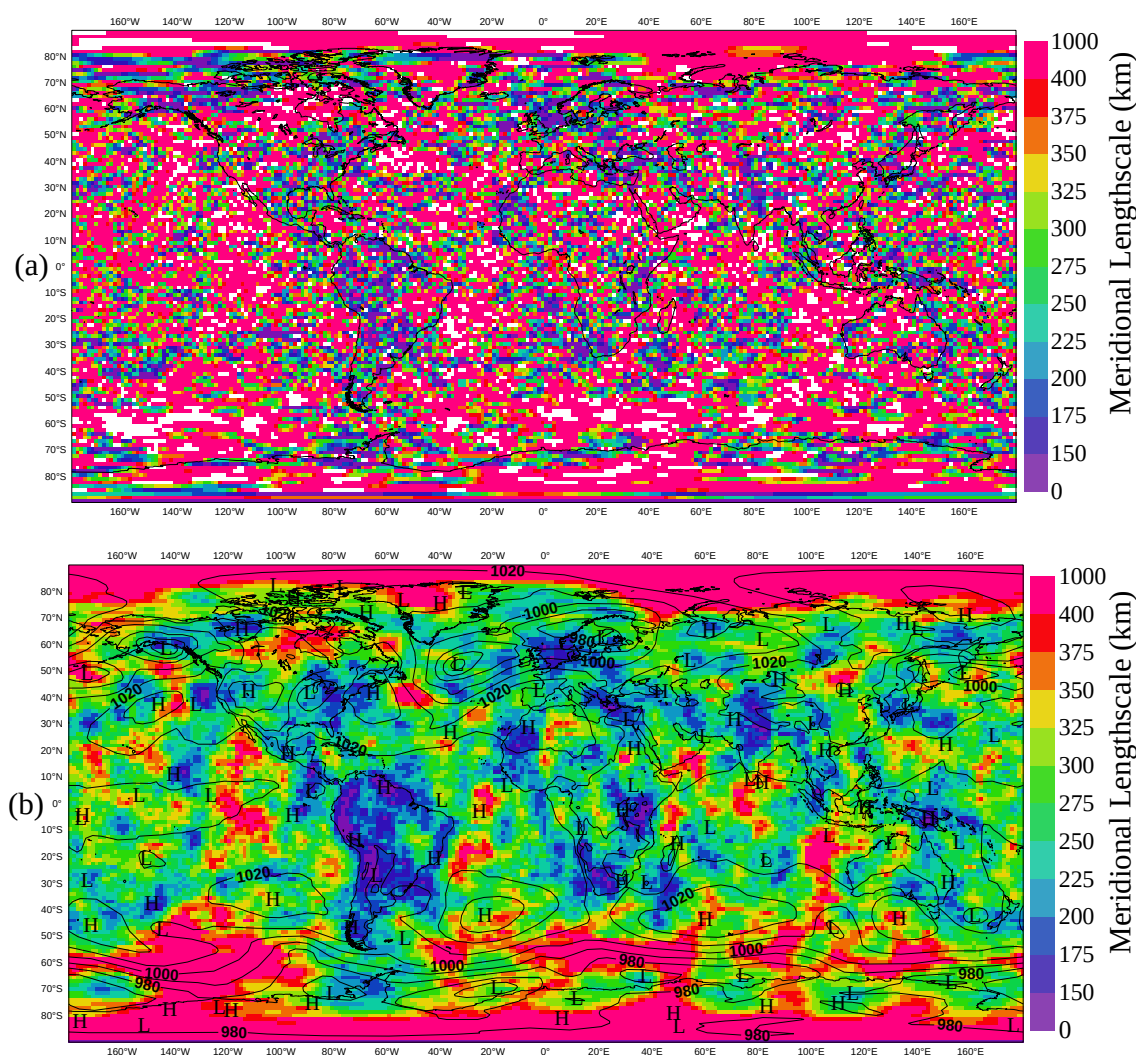
Figure 10: Meridional length-scales (km) for surface pressure on 10 February 2002 at 12 UTC. Top panel: raw length-scales. Bottom panel: wavelet-implied length-scales, superimposed on the background field of surface pressure.
